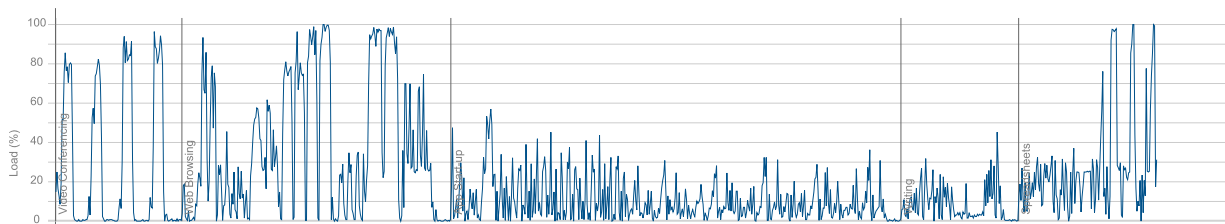
CPU Load (%)
